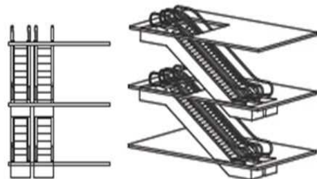
(6) PARALLEL NONCONTINUOUS
