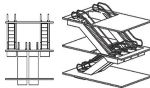
(5) PARALLEL CONTINUOUS
