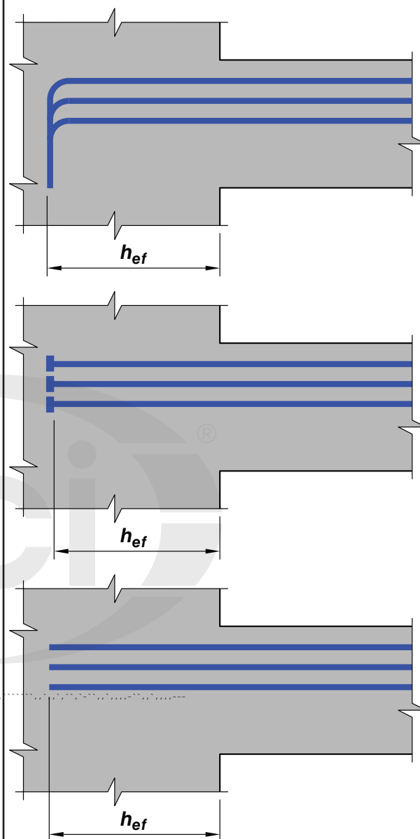
Fig. R2.3—Effective embedment depth for reinforcing bars for the purpose of determining concrete breakout strength.
