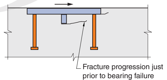
Fig. R17.11.1a—Examples of attachments with shear lugs.
