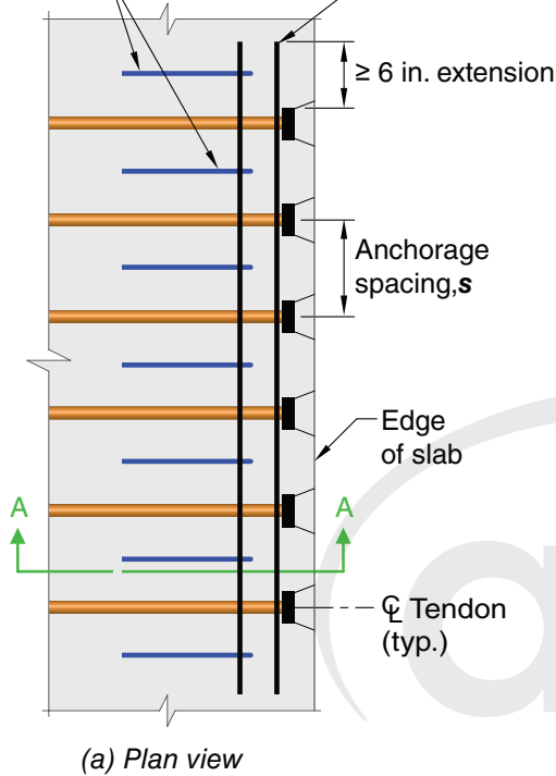
Fig. R25.9.4.4.6—Anchorage zone reinforcement for groups of 12.7 mm or smaller diameter tendons in slabs (other reinforcement not shown).
