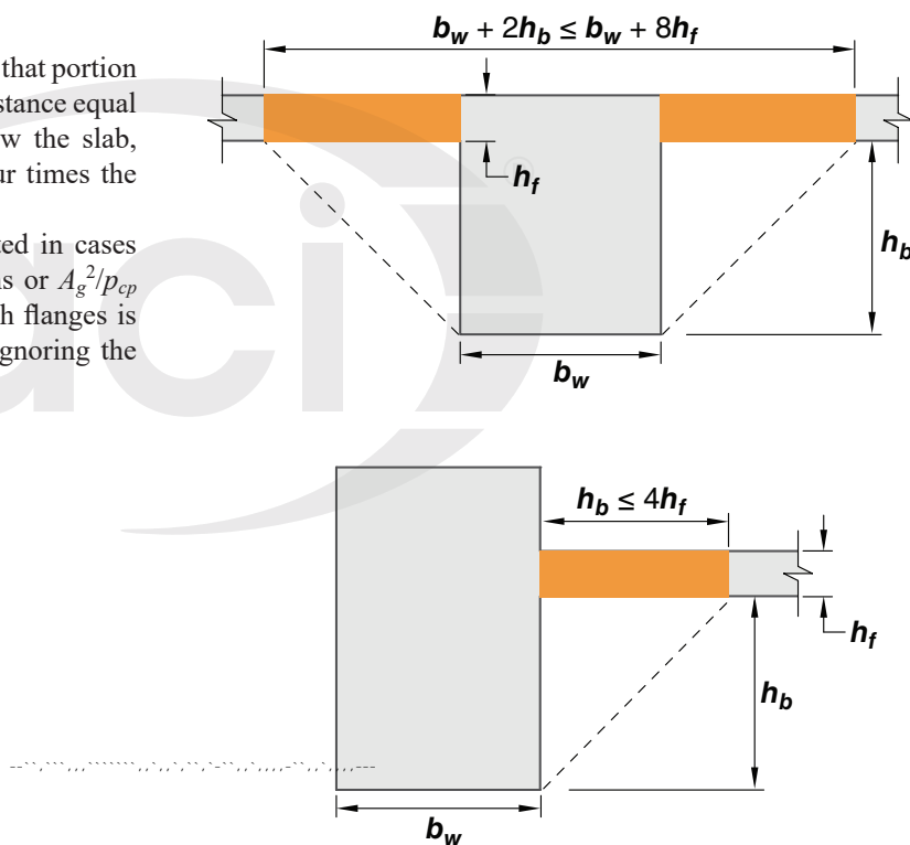
Fig. R9.2.4.4—Examples of the portion of slab to be included with the beam for torsional design.
