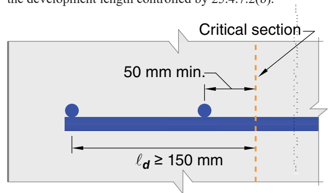
Fig. R25.4.7.2—Development of welded plain wire reinforcement.
