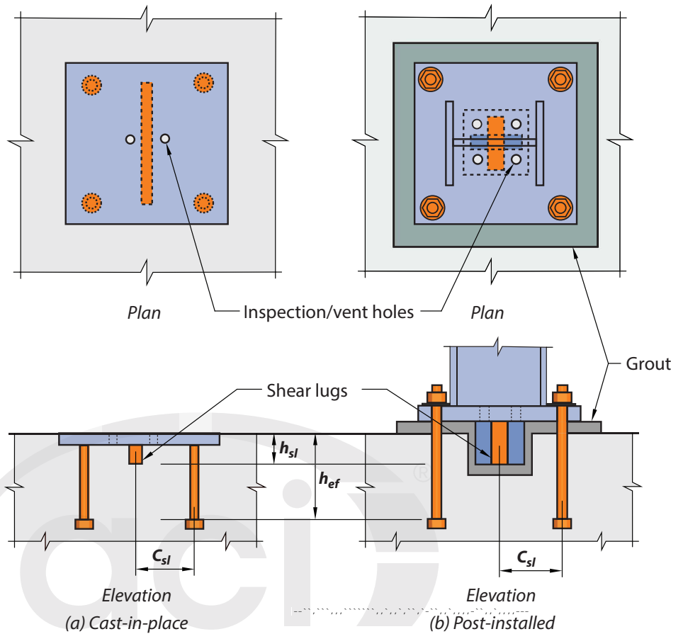
Fig. R17.11.1a—Examples of attachments with shear lugs.
