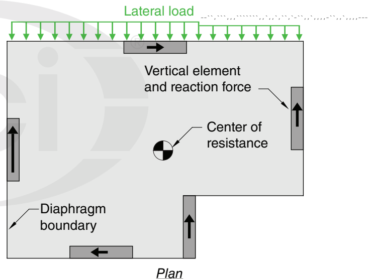
Fig. R12.4.2.3a—Example of diaphragm that might not be considered rigid in its plane.
