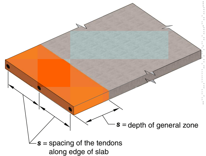
Fig. R25.9.4.1—Dimensions of general zone in post-tensioned slab.
