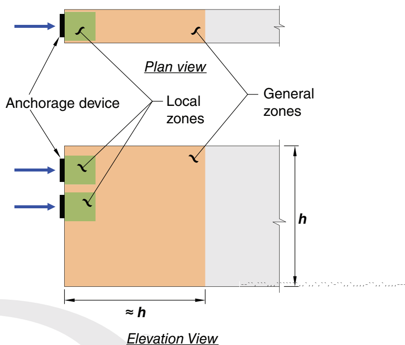
Fig. R25.9.1.1a—Local and general zones.
