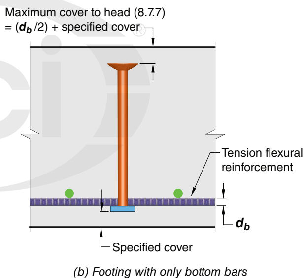
Fig. R20.5.1.3.6—Concrete cover requirements for headed shear stud reinforcement.
