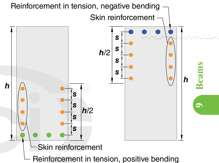
Fig. R9.7.2.3—Skin reinforcement for beams and joists with h > 900 mm.
