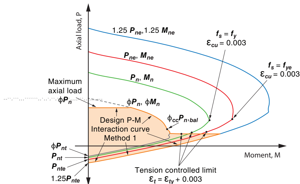
Fig. RB.11.3.3—P-M diagrams for Method 1.
