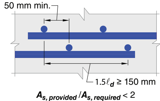
Fig. R25.5.4.1—Lap splices of plain welded wire reinforcement where A_{s,provided}/A_{s,required} < 2 .
