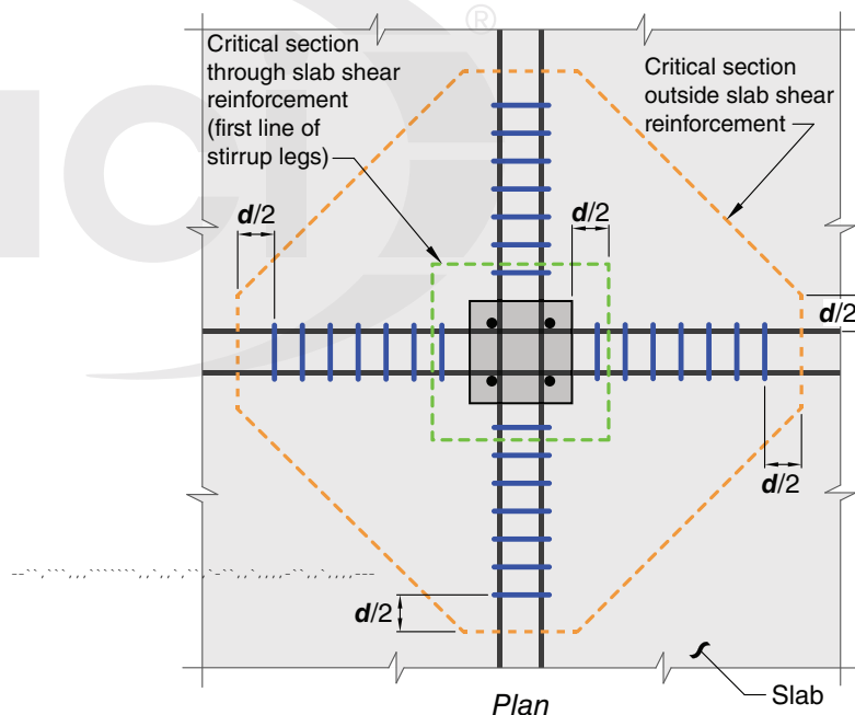
Fig. R22.6.4.2a—Critical sections for two-way shear in slab with shear reinforcement at interior column.
