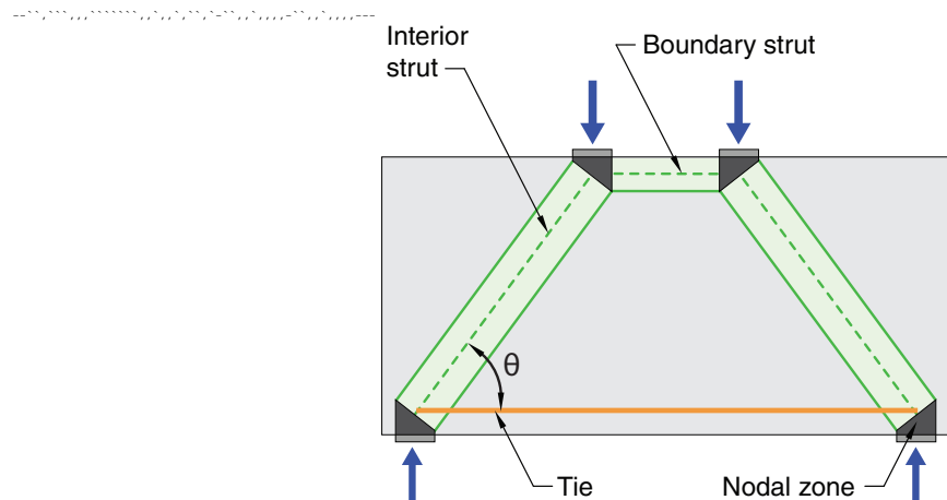
Fig. R23.2.1—Description of strut-and-tie model.
