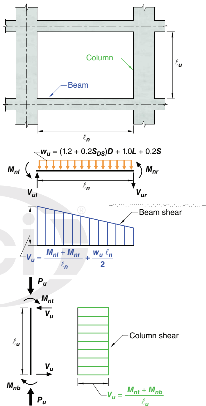
Fig. R18.4.2—Design shears for intermediate moment frames.
