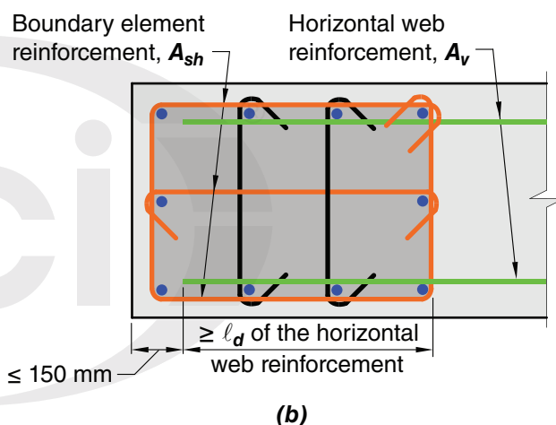
Fig. R18.10.6.4d—Development of wall horizontal reinforcement in confined boundary element.
