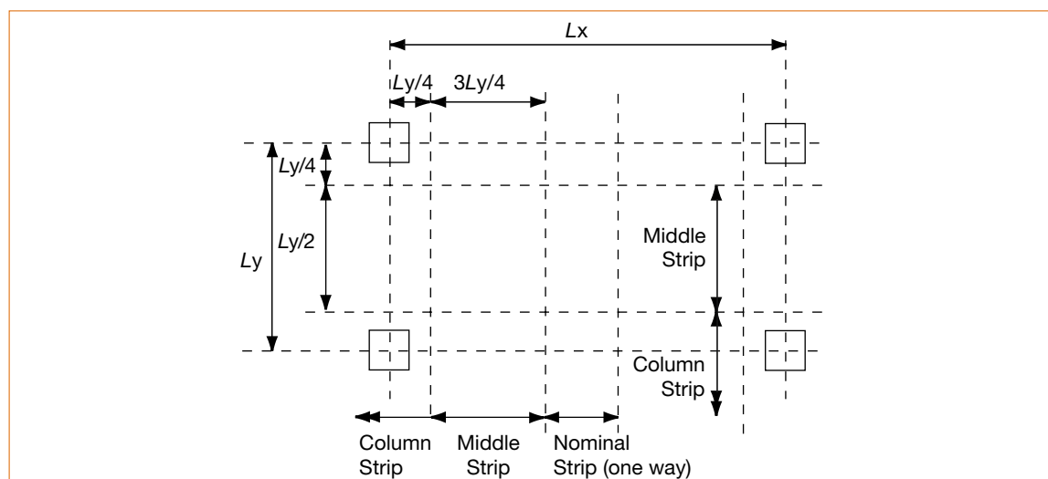
Figure 6.6 Division of reinforcement strips for flat slabs
