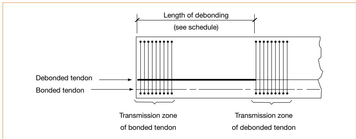
Figure 7.26 Transmission zones in pre-tensioned elements
