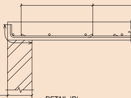
DETAIL 'B' (Slab depth less than 150)
