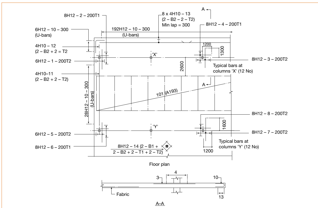
Figure 7.31 Example of untensioned reinforcement layout for an unbonded system
