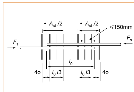
Figure 6.25 Links required for bursting at column laps
