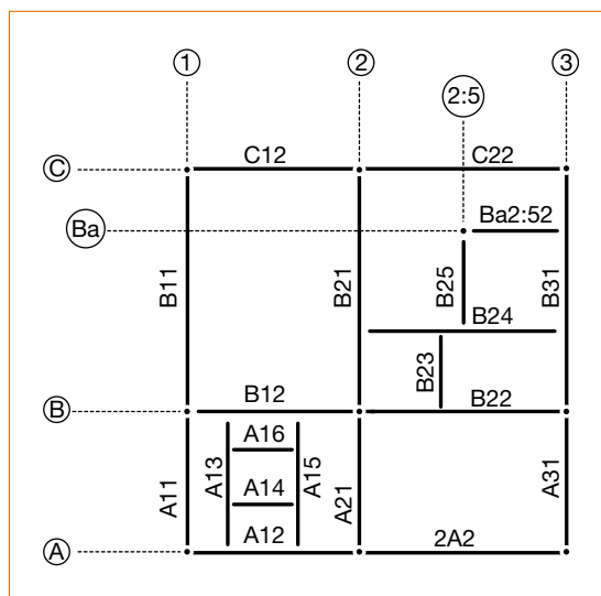
Figure 3.5 Framing plan
