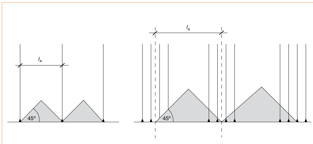
Figure 7.25 Unstressed zones near the edges of post tensioned floor slabs
