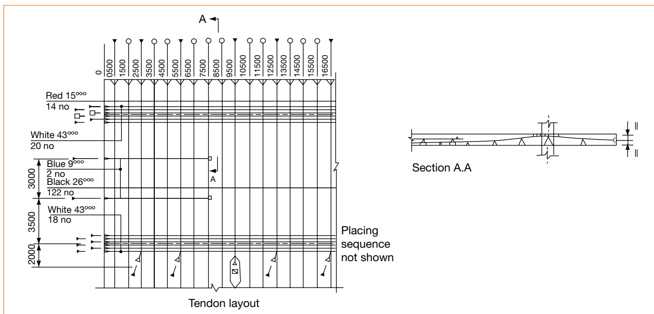
Figure 7.30 Typical unbonded tendon layout and placing sequence
