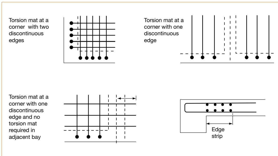
Figure 6.9 Torsion reinforcement at slab corners
