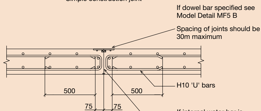
DETAIL 'A' Simple construction joint
