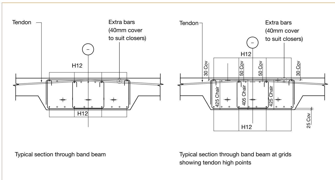
Figure 7.32 b) Typical tendon profile in a post-tensioned band beam and slab (typical sections)
