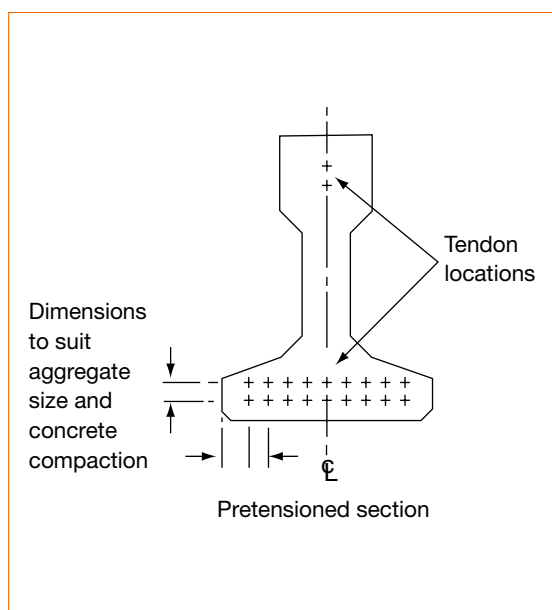
Figure 7.3 Symmetrical arrangement of tendons for pre-tensioned units
