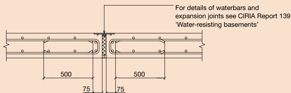
DETAIL 'C' Movement joint
