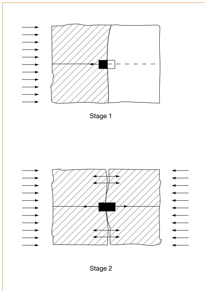
Figure 7.24 Tensile forces at anchorage coupling
