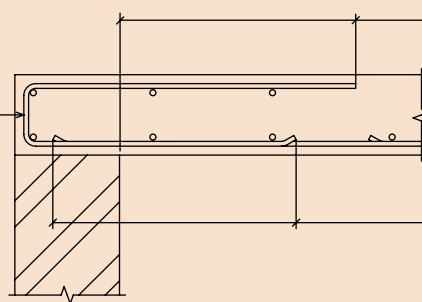
DETAIL 'A' (Slab depth 150 or greater)
