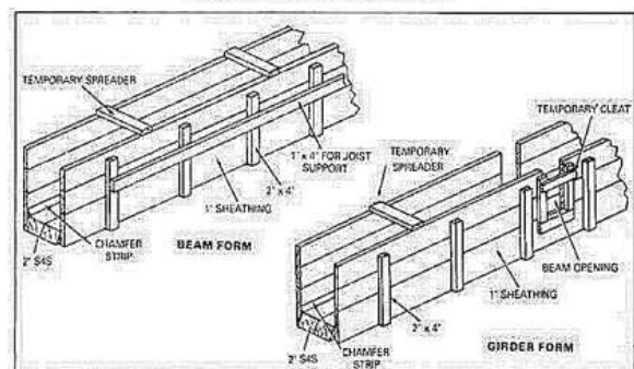
Figure 5-12. Beam and girder forms
