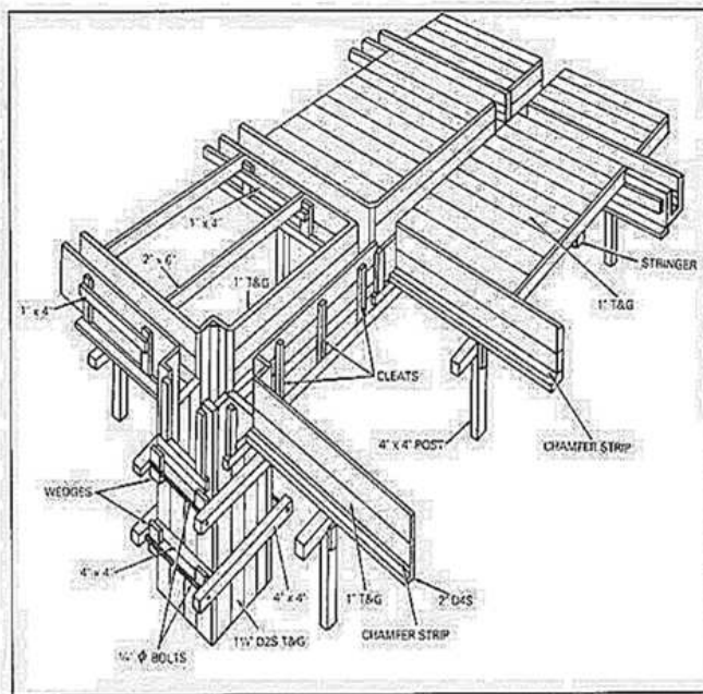
Figure S-13. Beam, column and floor form
