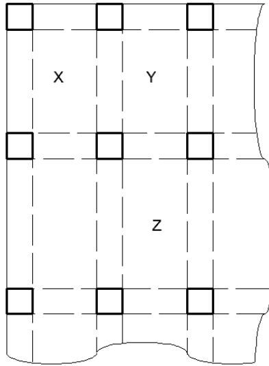
fig 2. plan of typical to-way slab floor with beams on column lines
